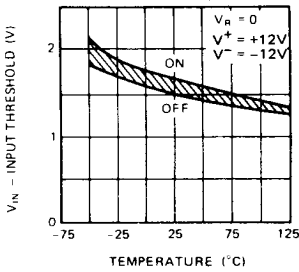
V_{IN} THRESHOLD vs TEMPERATURE
