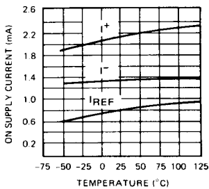
ON SUPPLY CURRENT vs TEMPERATURE
