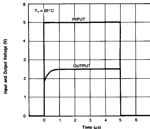
Figure 9. Pulse Response
