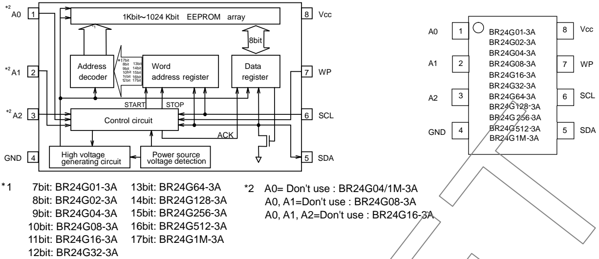
Fig.2 Block diagram
