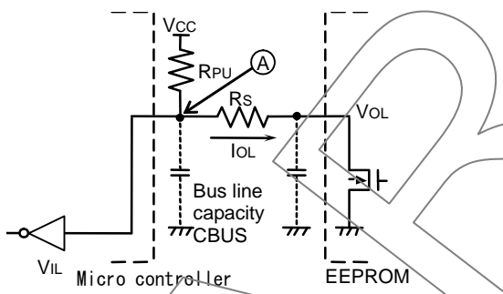
Fig.55 I/O Circuit Diagram
