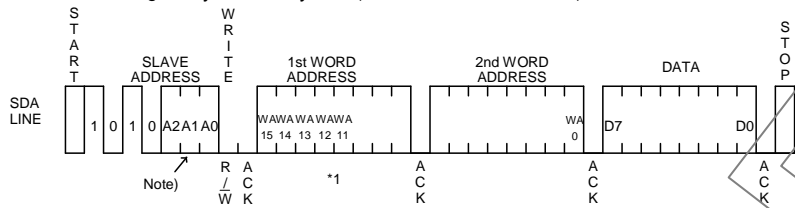
Fig.39 Byte write cycle (BR24G32/64/128/256/512/1M-3A)
