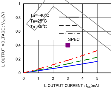
Fig.6 'L' output voltage V_{OL2-I_{OL}} ( V_{cc}=2.5V )
