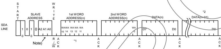
Fig.41 Page write cycle (BR24G32/64/128/256/512/1M-3A)
