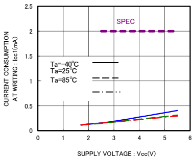
Fig.9 Current consumption at WRITE operation I_{cc1} (fsc1=1MHz BR24G01/02/04/08/16/32/64-3A)
