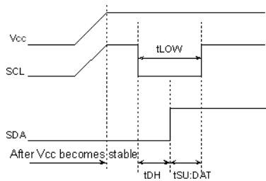
Fig.60 When SCL='H' and SDA='L'
