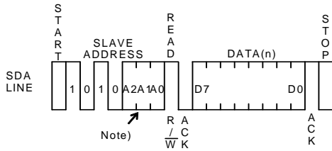
Fig.45 Current read cycle
