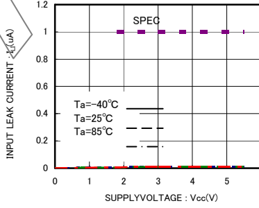
Fig.7 Input leak current I_I (A0,A1,A2,SCL,WP)
