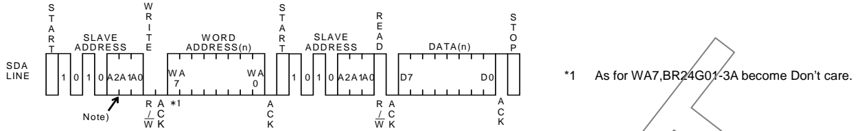
Fig.43 Random read cycle (BR24G01/02/04/08/16-3A)
