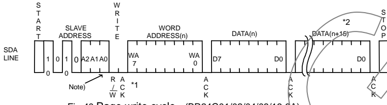
Fig.40 Page write cycle (BR24G01/02/04/08/16-3A)
