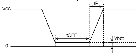
Fig.59 Rise waveform diagram
