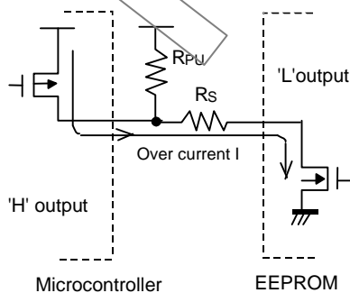
Fig.56 I/O circuit diagram
