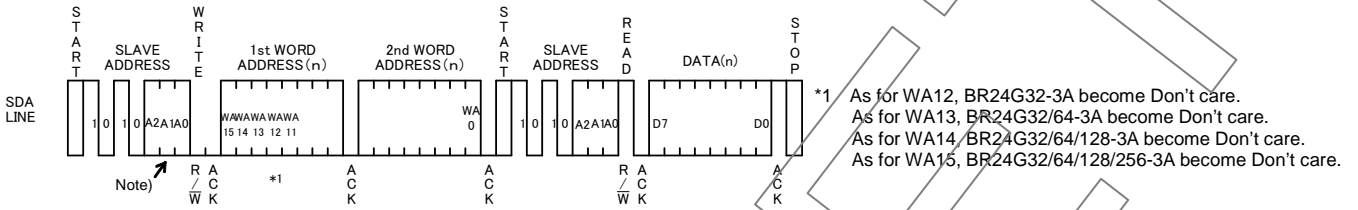
Fig.44 Random read cycle (BR24G32/64/128/256/512/1M-3A)
