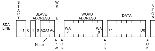
Fig.38 Byte write cycle (BR24G01/02/04/08/16-3A)
