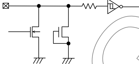
Fig.58 Input / output pin circuit diagram
