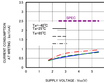
Fig.10 Current consumption at WRITE operation I_{cc1} (fsc1=1MHz BR24G128/256-3A)
