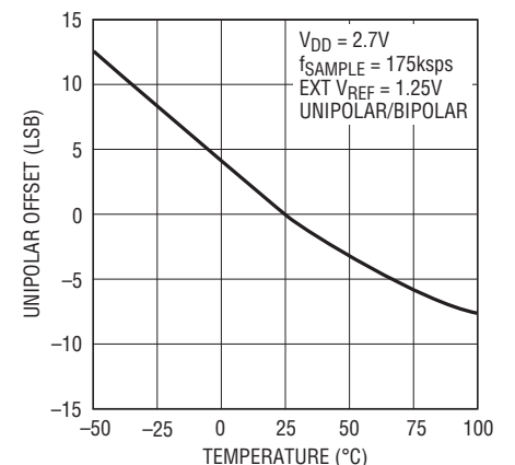
Gain Error Drift (LTC1867L) vs Temperature
