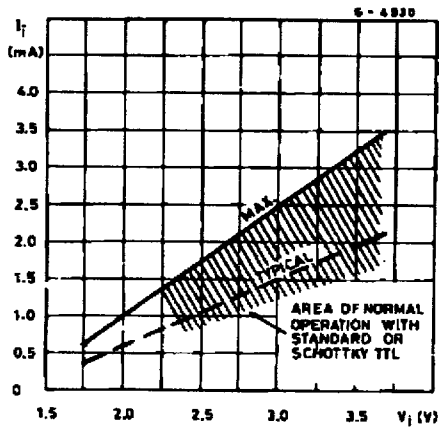
Figure 16 : Input Current as a Function of Input Voltage (for ULN2805A)
