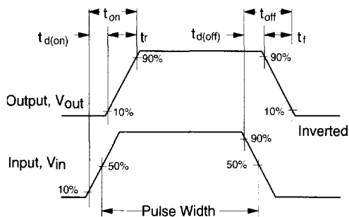
Figure 12. Switching Waveforms.
